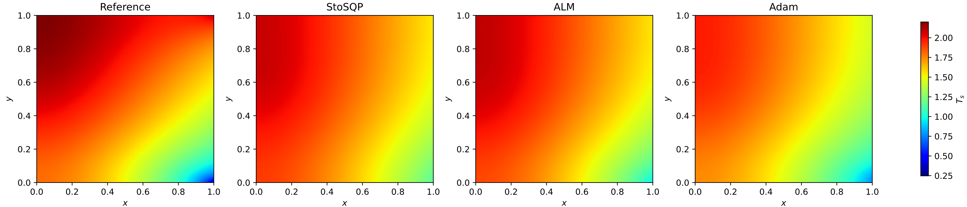
Final-time fuel temperature field T_s at t = 1.000
